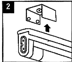
2) SNAP LIGHT FIXTURE INTO BRACKET
