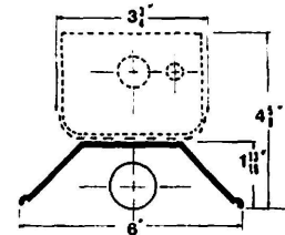
WELDED REF 12 ONE LIGHT SLIMLINE PAN WITH SYMMETRIC REFLECTOR
