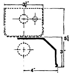
WELDED REF 11 ONE LIGHT SLIMLINE PAN WITH ASSYMMETRIC REFLECTOR
