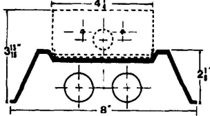
REF 9 ONE OR TWO LIGHT WITH NARROW SYMMETRIC REFLECTOR
