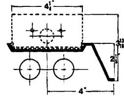
REF 8 ONE OR TWO LIGHT WITH ASSYMMETRIC REFLECTOR
