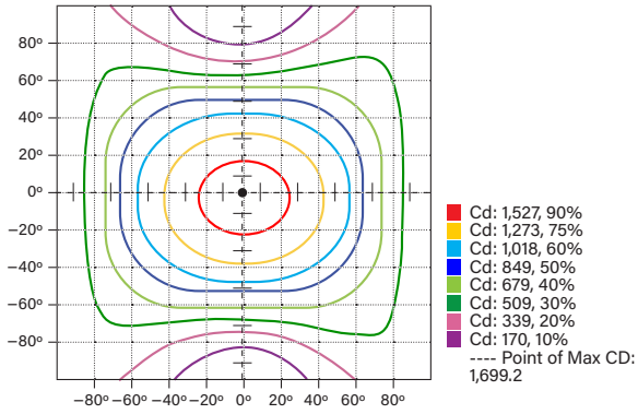
ISOCANDELA PLOT
